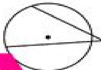
Two Secants
