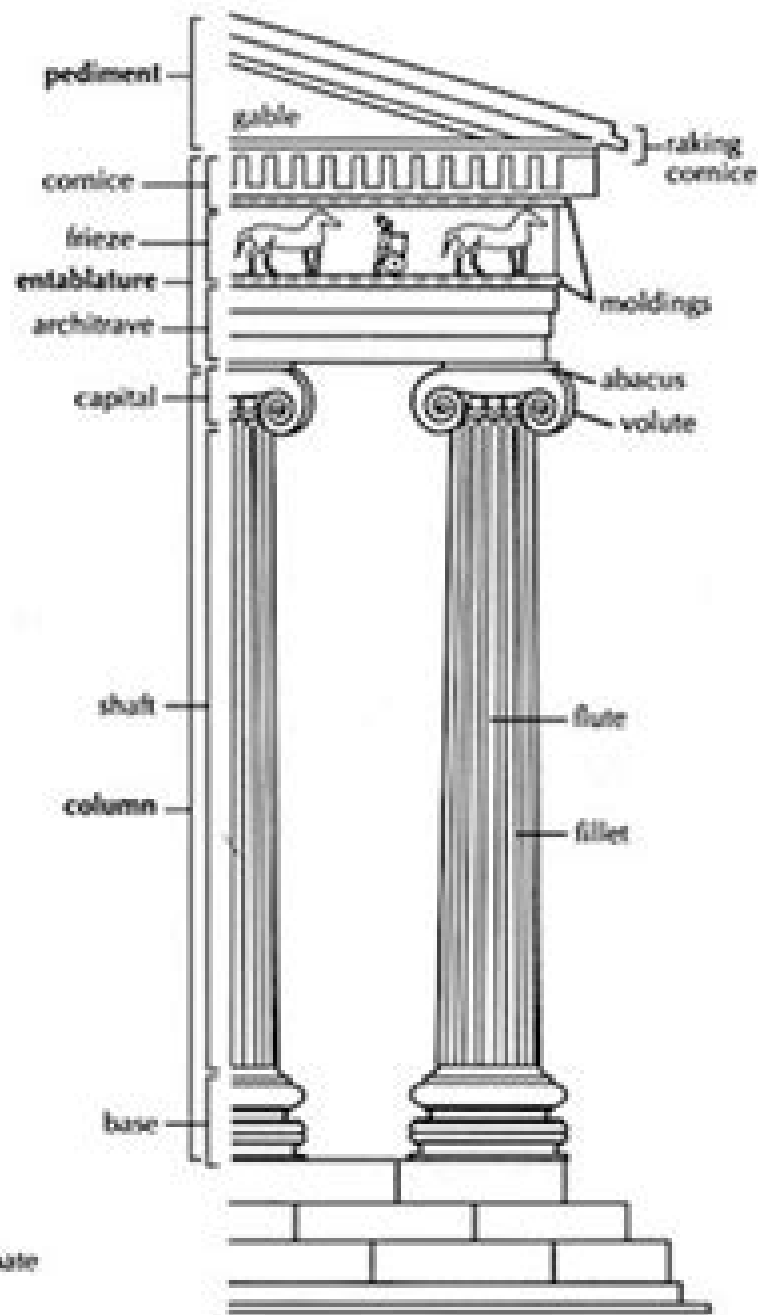
Ionic order
