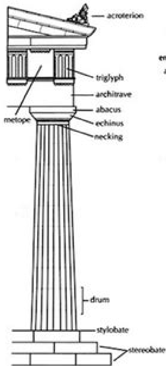
Doric order
